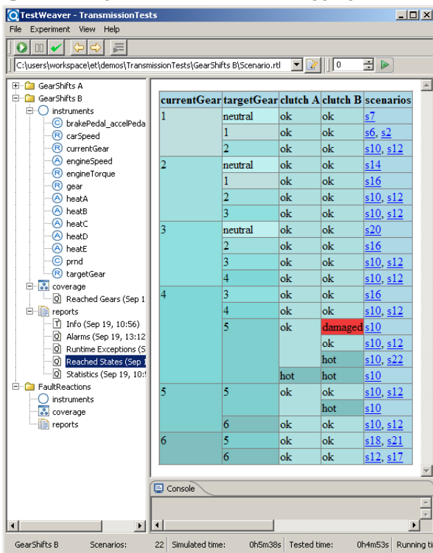
Figure 9: TestWeaver displaying a coverage report
